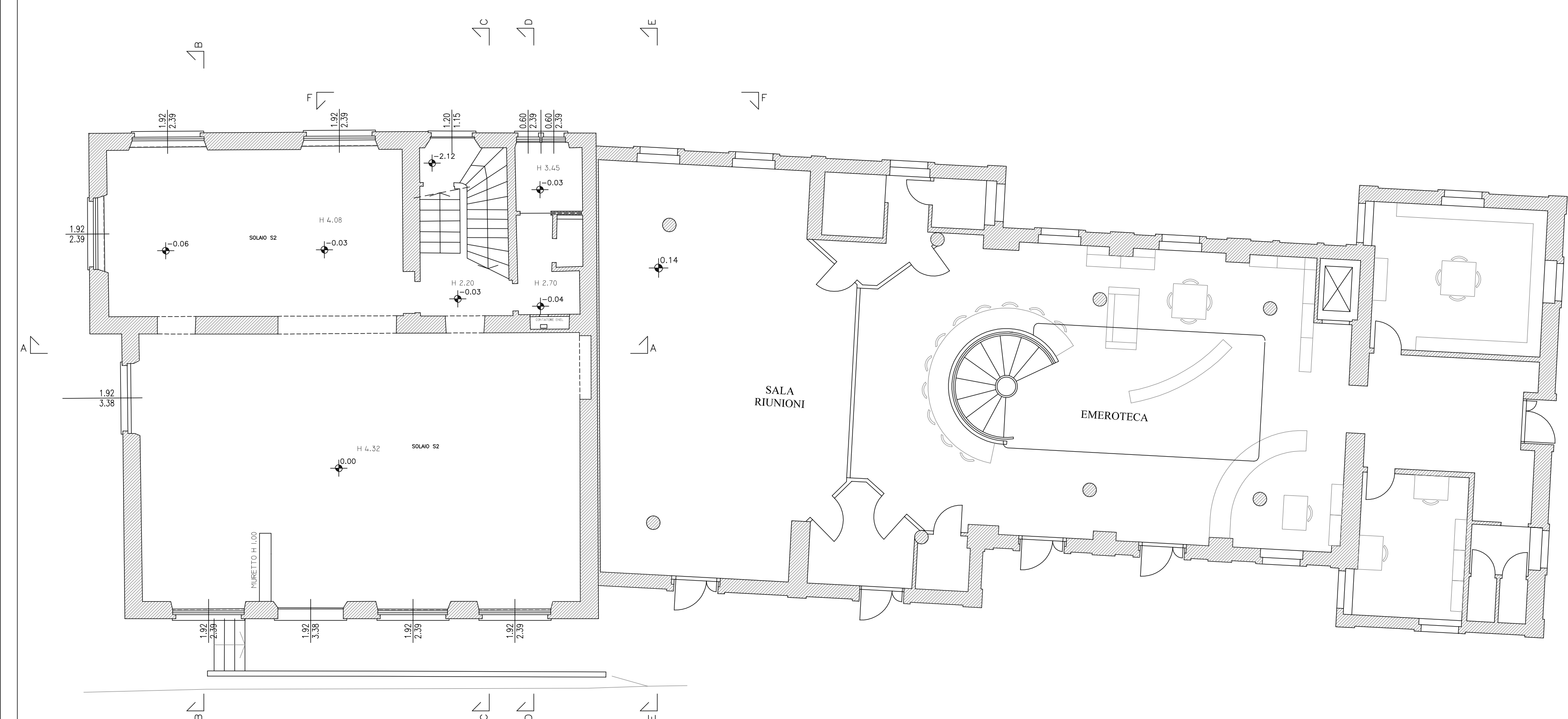
PIANO TERRA
